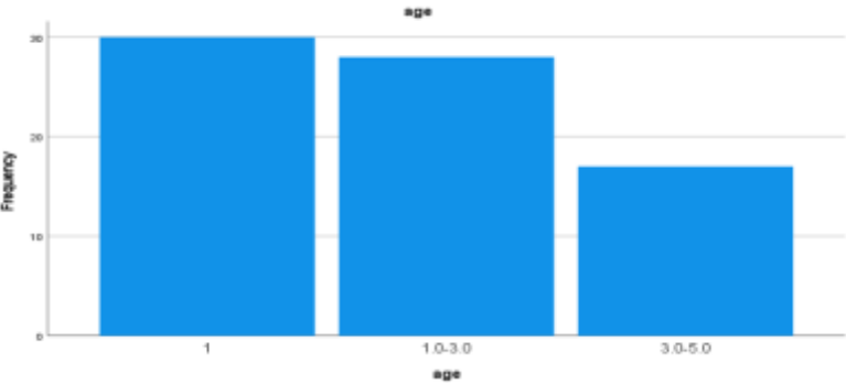
GRAPH-1: The frequency distribution of the variable “Age” in different categories
