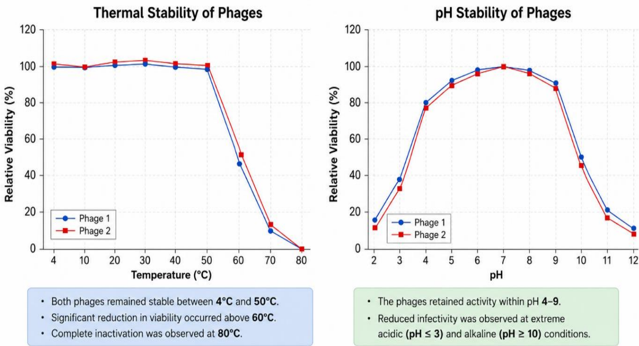
Figure 3: pH and thermal stability of EcoPhage1 and EcoPhage2
